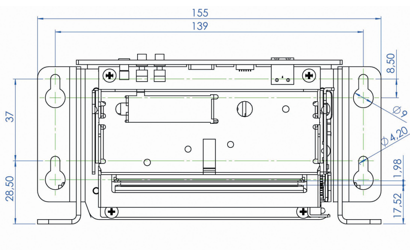
Drawing 2: GeBE-COMPACT for 82 mm paper width
